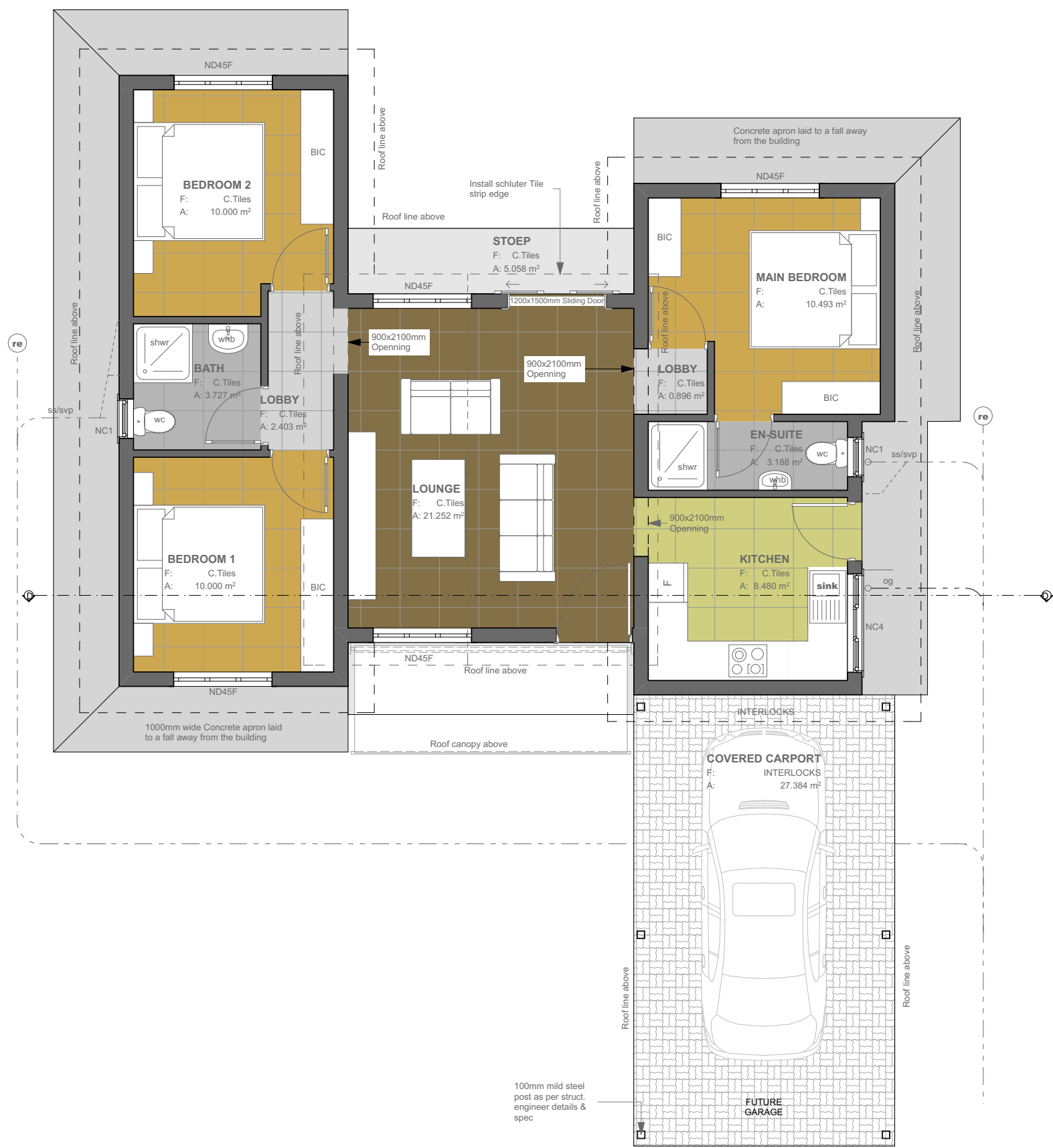
TOTAL BUILDING AREA = 84.77m 2 GROUND FLOOR PLAN
